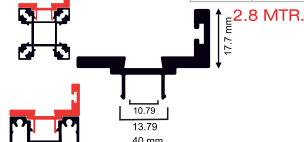
Portal Rebate
