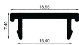
Portal Cap
