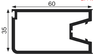
Stile Door Fix Profile
