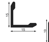
Corner Guard-15mm / 19mm
