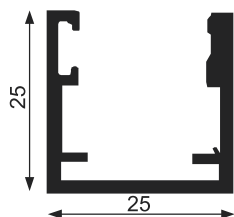
Fix Profile
