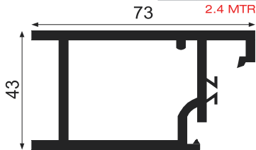
Stile Door Male Profile
