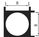
90° Section-8mm
