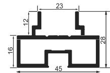
Door Profile Top And Bottom
