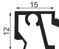
Block Fix M/f Profile
