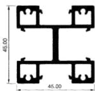
Portal 45
