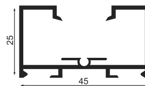
Fix Profile
