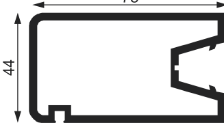
Stile Door Fix Profile
