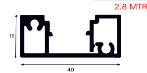
Fix M/f Profile
