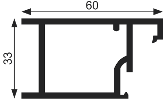
Stile Door Male Profile
