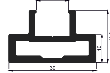
Vertical Profile
