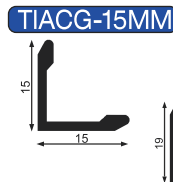
Corner Guard-15mm / 19mm
