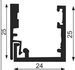
Fix M/f Profile
