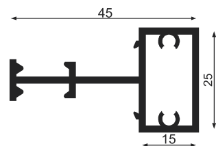
Block Fix M/f Profile
