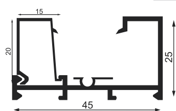
Fix M/f Profile
