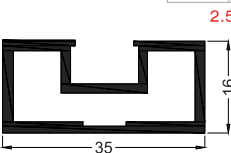
Vertical Profile
