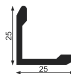
Corner Guard-25mm
